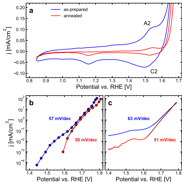
Figure 3: Electrochemical response of a \text{Co}_3\text{O}_4(111) film in 0.1 M NaOH before and after annealing at 400^\circ\text{C} in Ar. The measurements were performed on a RDE at 3000 rpm. (a) Cyclic voltammogram measured at 5\text{ mV/s} , showing the capacitive potential range. (b,c) Tafel plots of the OER current density. The data correspond to (b) the steady state current density, obtained by stepwise increase of the potential every 4 min and (c) the current density during anodic potential sweeps at 5\text{ mV/s} .
