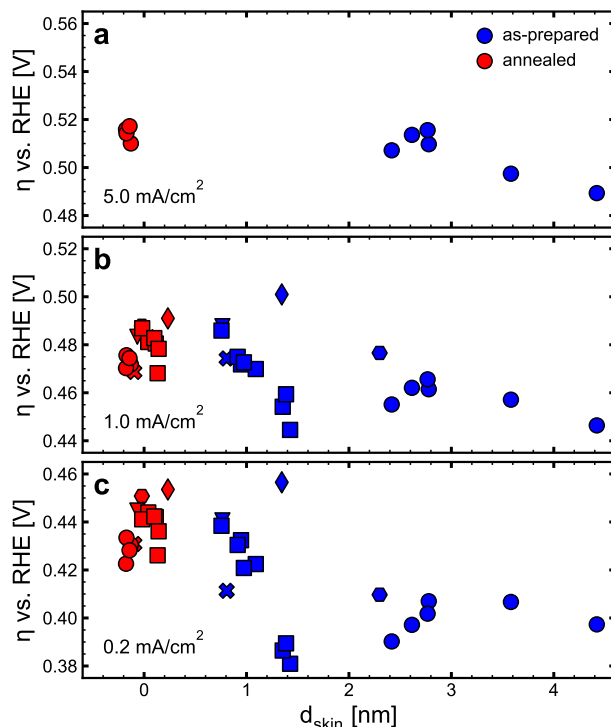
Figure 6: Correlation of the skin layer thickness with the OER activity of different \text{Co}_3\text{O}_4(111) films. The average thickness \langle d_{\text{skin}} \rangle was obtained from the operando SXR data, the OER overpotentials at 0.2 \text{ mA/cm}^2 , 1 \text{ mA/cm}^2 and 5 \text{ mA/cm}^2 from the anodic sweeps of the simultaneously recorded CVs.
